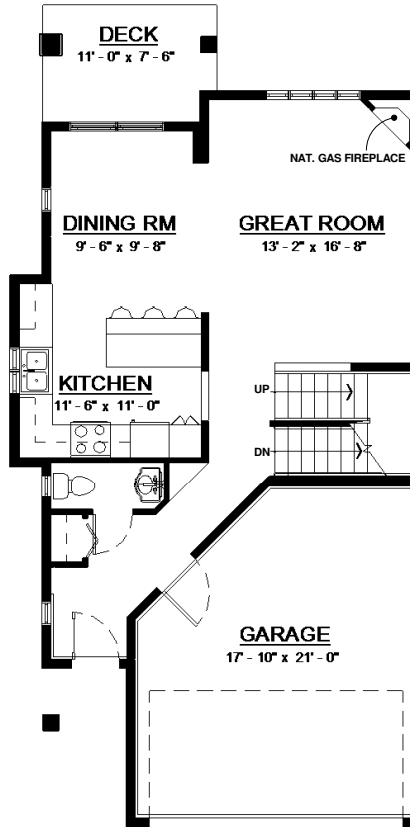
B1 - MAIN FLOOR PLAN
