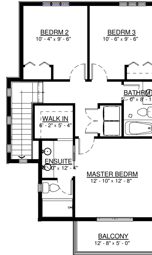
A1 - UPPER FLOOR PLAN
