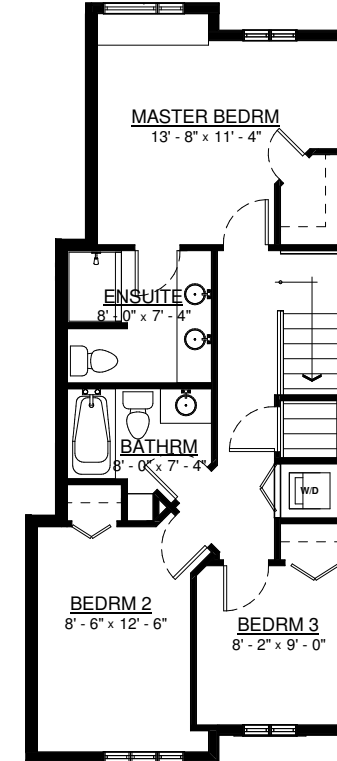
A3 - UPPER FLOOR PLAN
