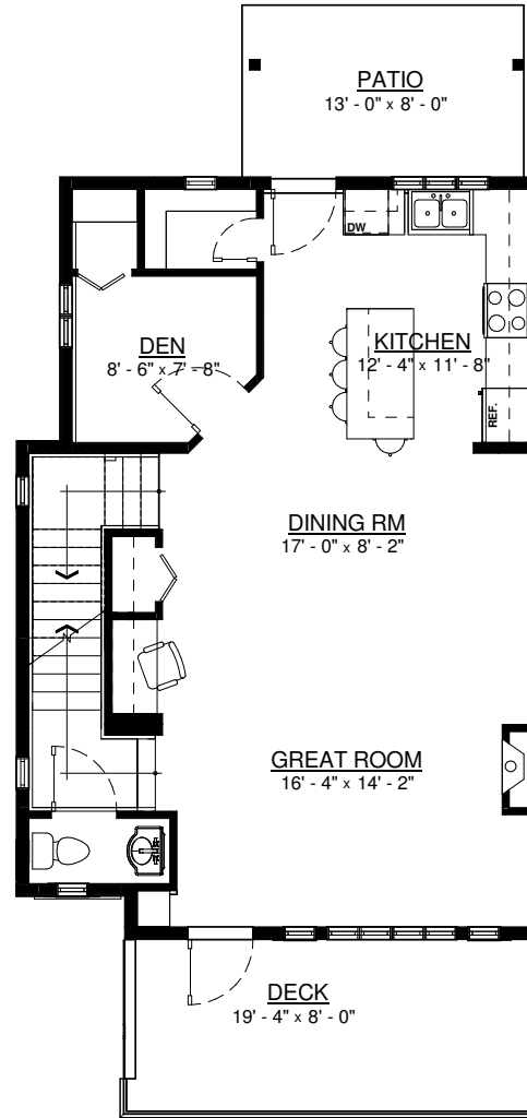
A1 - MAIN FLOOR PLAN
