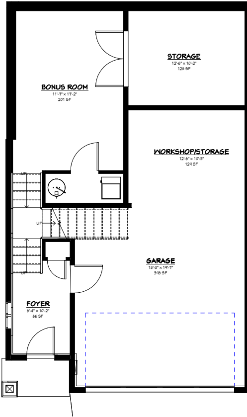
BASEMENT 561 SQ FT NOT INCLUDING GARAGE MECHANICAL ROOM UNFINISHED (27 SQ.FT.)
