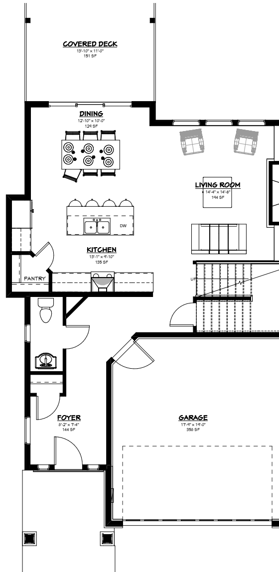
MAIN FLOOR 836 SQ FT
