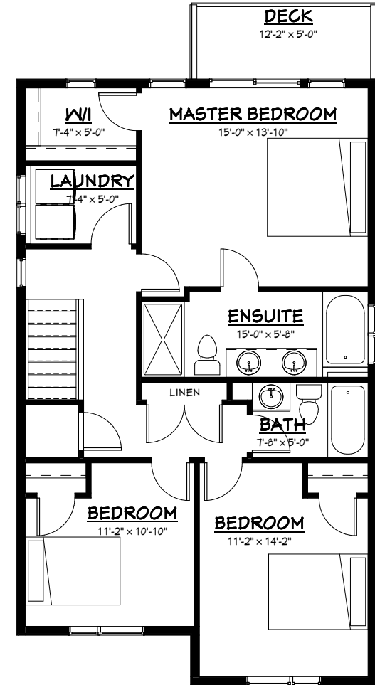
2nd FLOOR 872 SQ. FT. FINISHED NOT INC. STAIRS
